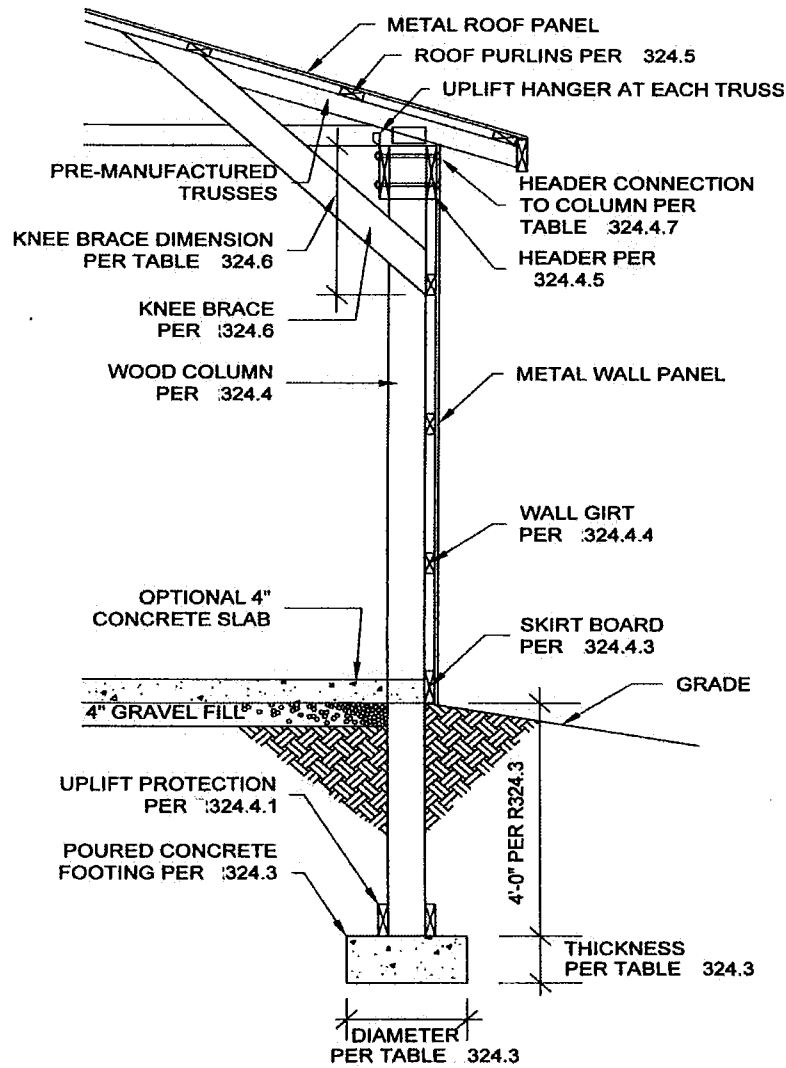
FIGURE 324 POST AND FRAME WALL SECTION. (NO SCALE)
