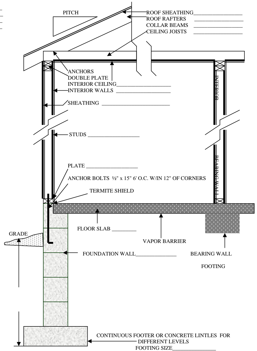
X-SECTIONS FOR STRUCTURES W/O CELLAR, BASEMENT, OR CRAWL SPACE
